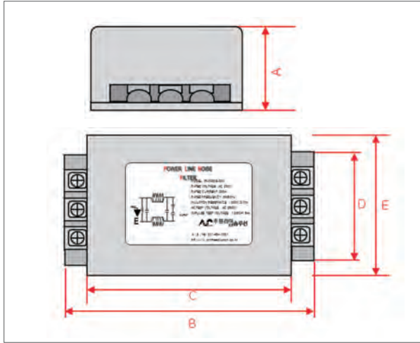
< Three Phase Filter >
