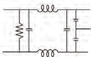
Single-Phase
