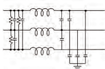
3-Phase
